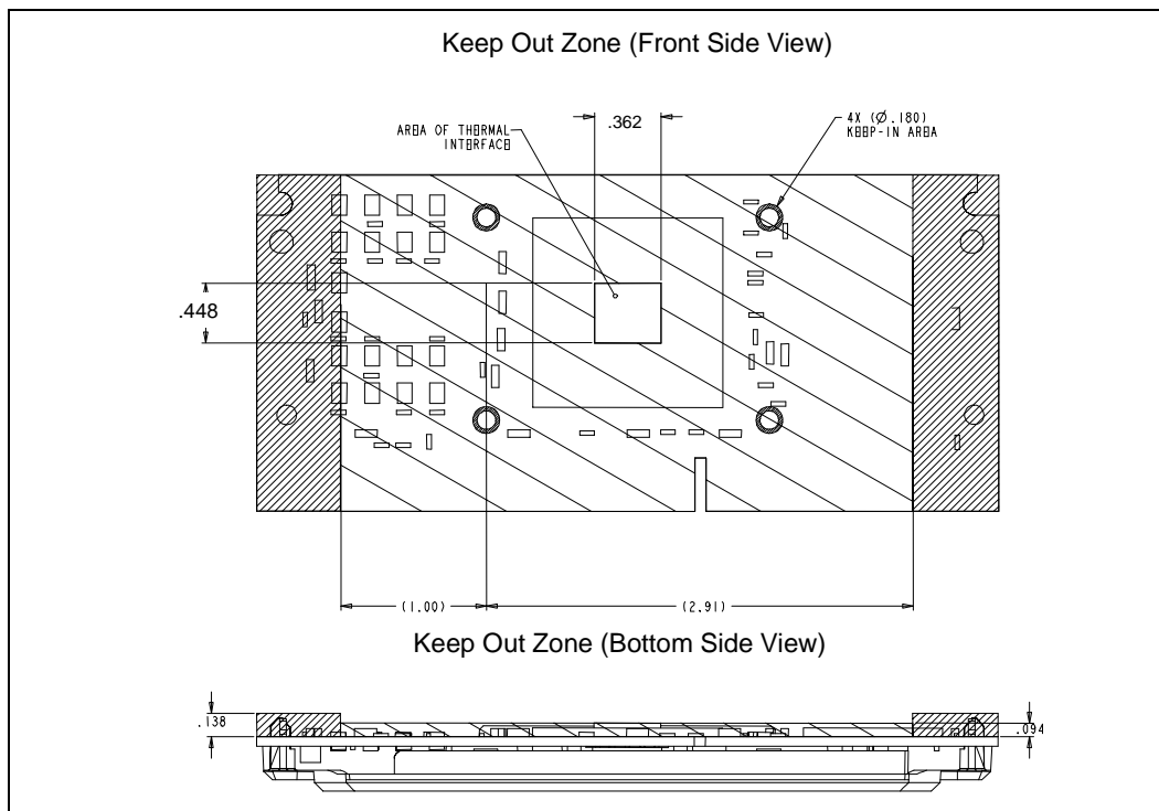
Figure 43. S.E.C.C.2 Packaged Processor Substrate (CPIUD 068xh) — Keep-Out Zone
