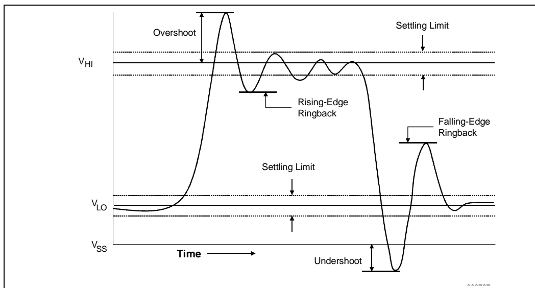
Figure 17. Signal Overshoot/Undershoot, Settling Limit, and Ringback 1
