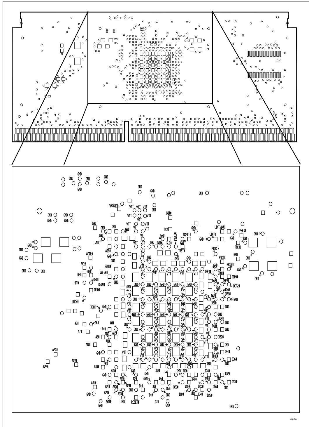
Figure 49. Intel® Pentium® III Processor S.E.C.C. 2 Via Map
