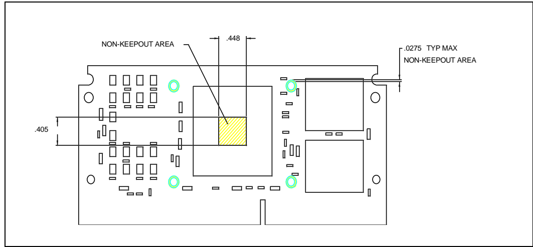
Figure 41. S.E.C.C.2 Packaged Processor Substrate (CPUID 068xh) — Keep In Zones
