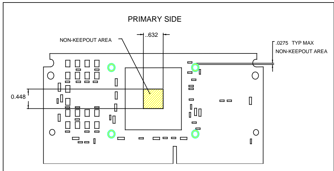
Figure 41. S.E.C.C.2 Packaged Processor Substrate (CPUID 068xh) — Keep In Zones
