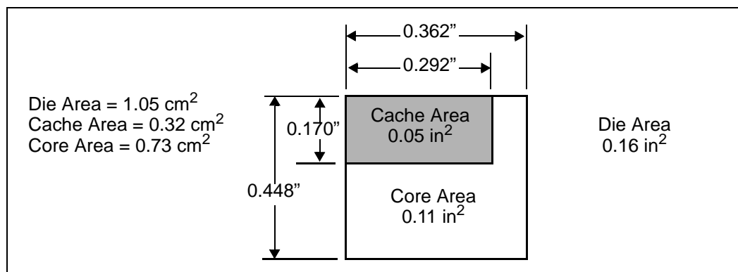
Figure 21. Processor Functional Die Layout (up to CPUID 0683h)
