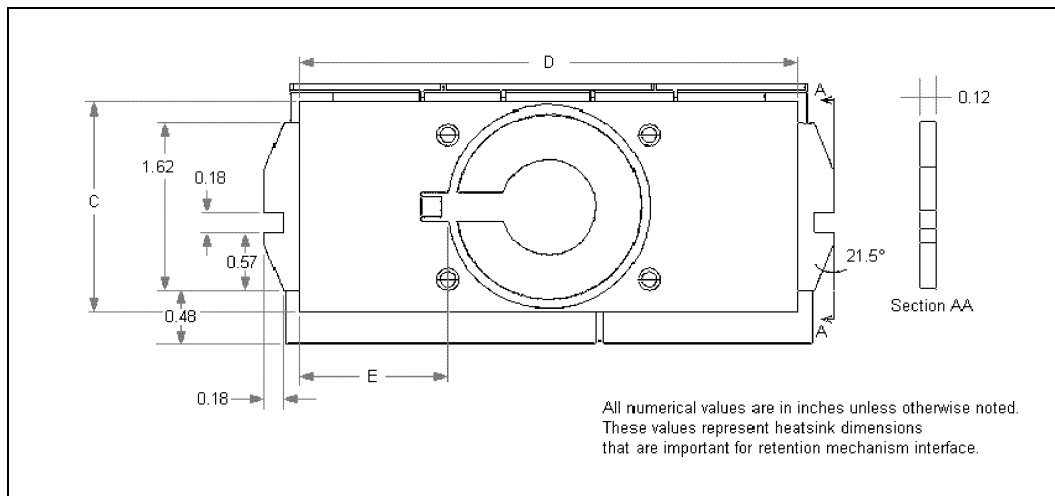
Figure 52. Front View Space Requirements for the Boxed Processor with S.E.C.C.2 Packaging
