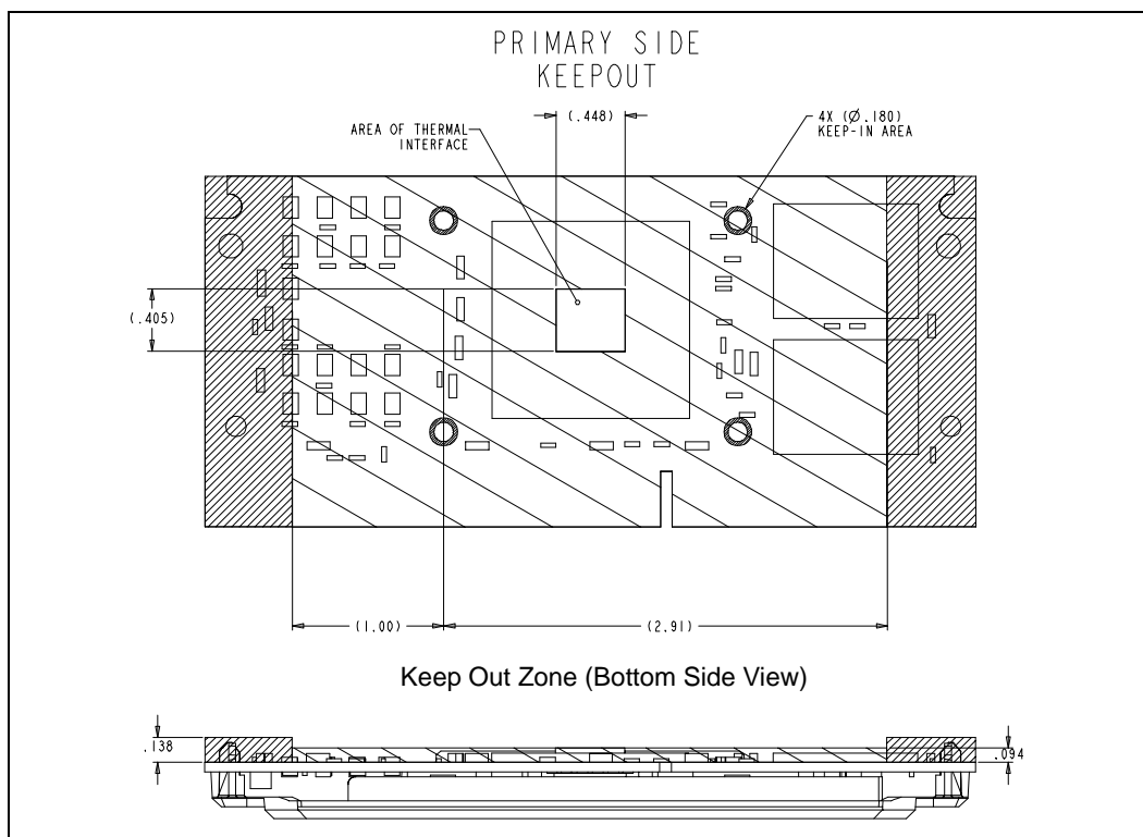
Figure 43. S.E.C.C.2 Packaged Processor Substrate (CPIUD 068xh) — Keep-Out Zone
