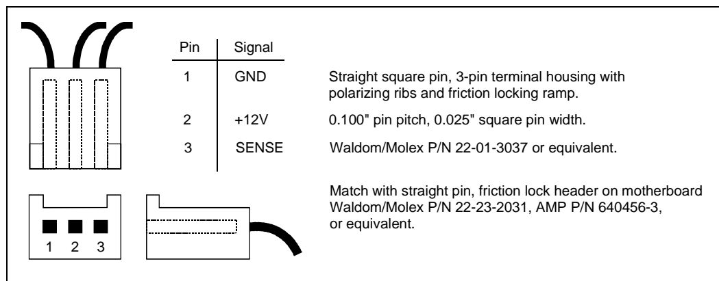
Figure 54. Boxed Processor Fan Heatsink Power Cable Connector Description
