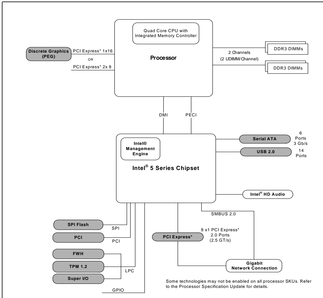
Figure 1-1. Intel® Core™ i7-800 and i5-700 Desktop Processor Series Platform Diagram
