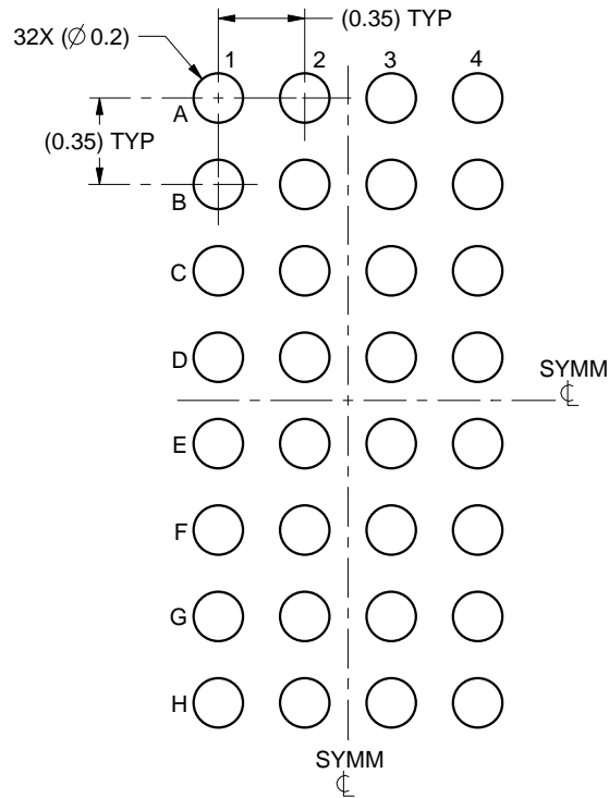
LAND PATTERN EXAMPLE SCALE:30X
