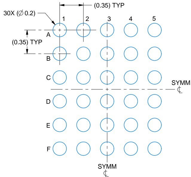
LAND PATTERN EXAMPLE SCALE:30X
