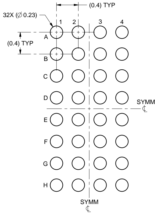
LAND PATTERN EXAMPLE SCALE:25X
