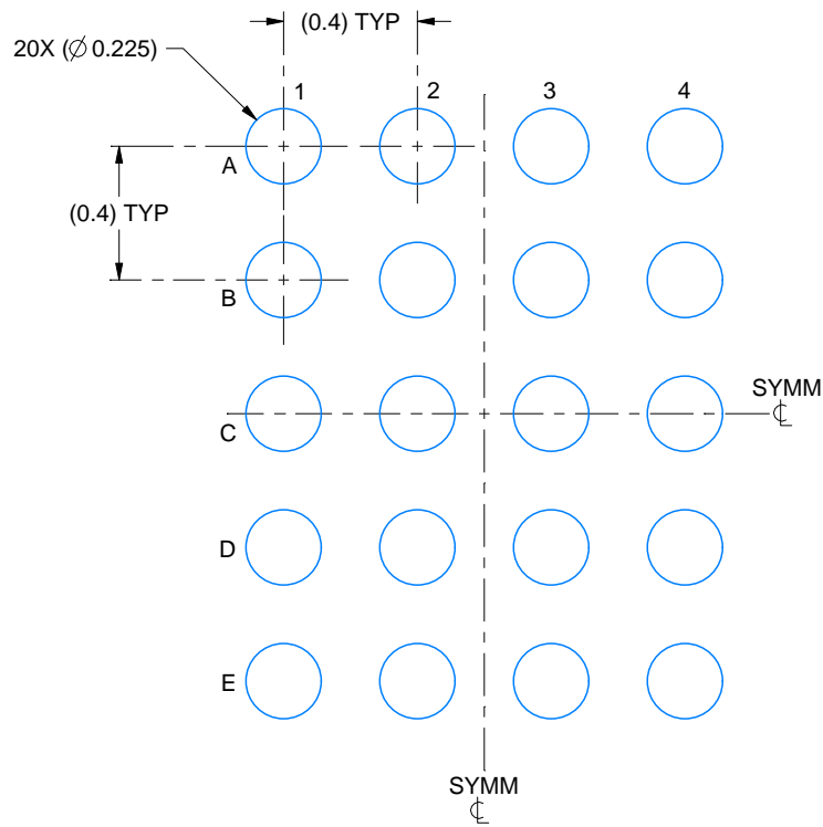
LAND PATTERN EXAMPLE EXPOSED METAL SHOWN SCALE:40X
