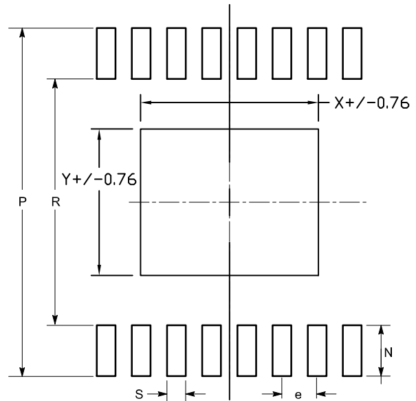
LAND PATTERN
