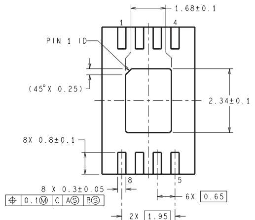
BOTTOM SIDE OF PACKAGE
