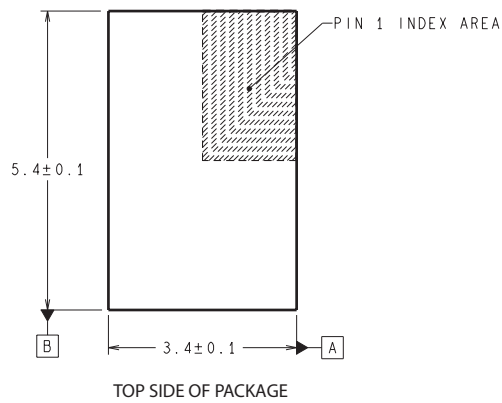
TOP SIDE OF PACKAGE
