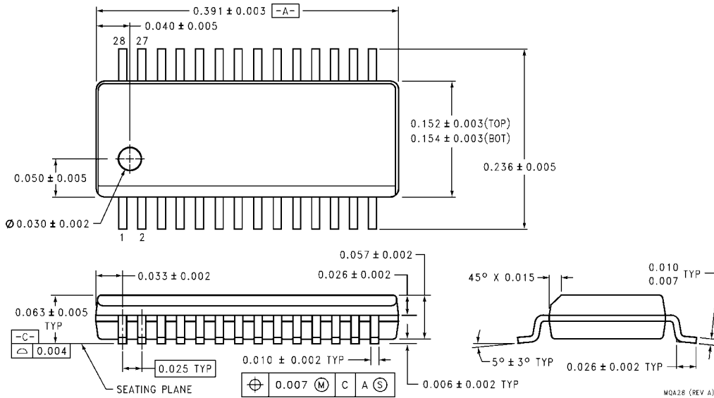
28-Lead Quarter Size Outline Package (QSOP), JEDEC MO-137, 0.150" Wide Package Number MQA28
