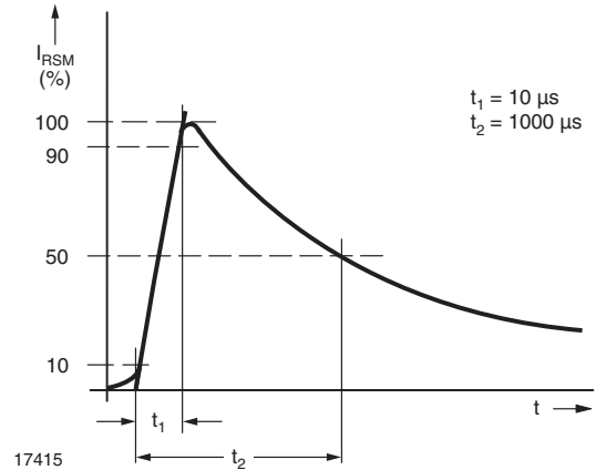
Fig. 4 - Pulse Waveform
