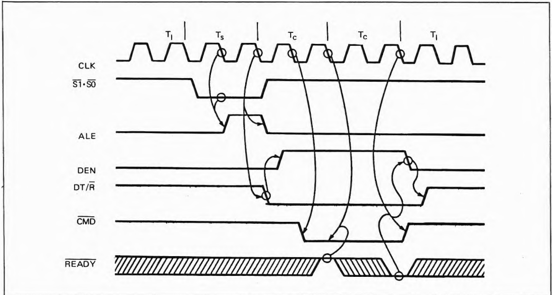
Figure 7. Idle-Read-Idle Bus Cycles with MB = "1".
