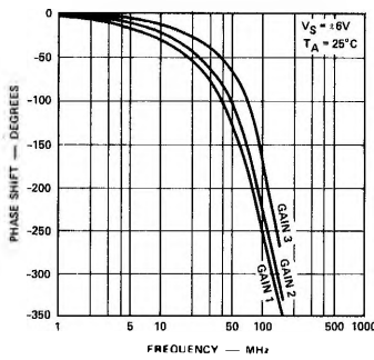
PHASE SHIFT AS A FUNCTION OF FREQUENCY
