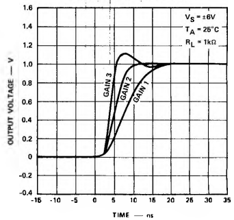
PULSE RESPONSE
