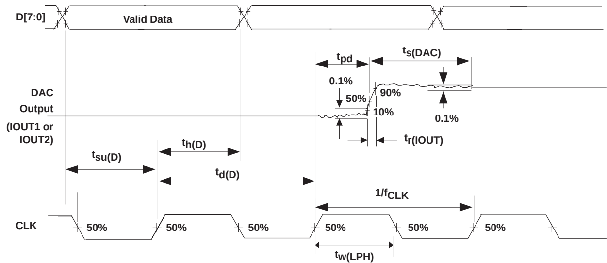
Figure 23. Timing Diagram
