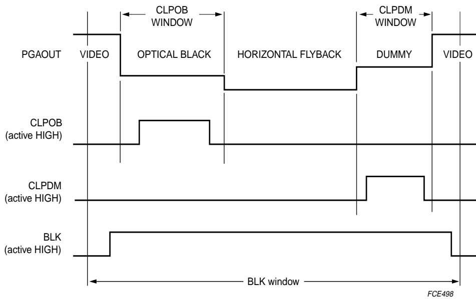
Fig.6 Line frequency timing diagram.
