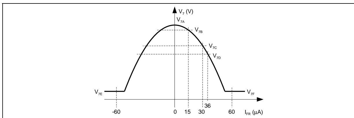
Figure 2 : Parabola Characteristics
