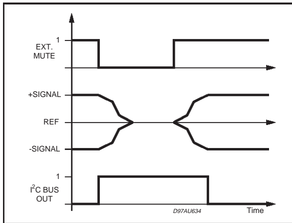
Figure 5. Softmute Timing
