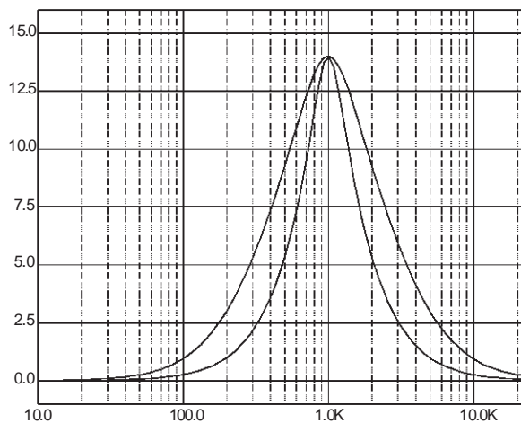
Figure 12. Mid Q-factor @ fc=1kHz, Gain=14dB
