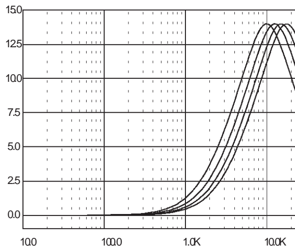
Figure 14. Treble Center Frequencies @ Gain = 14dB
