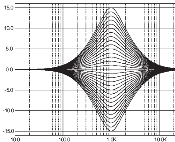
Figure 10. Mid Control @ fc=1kHz, Q=1
