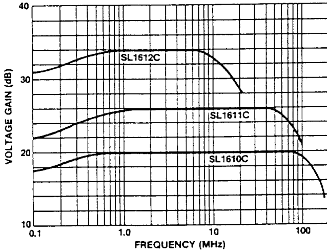
Fig 8 Typical voltage gain ( R_S=50\Omega )
