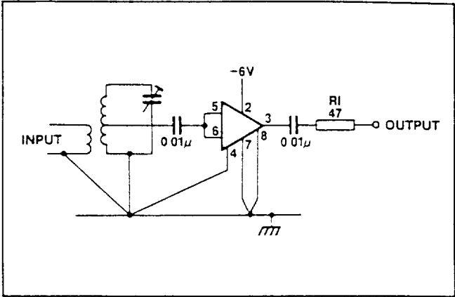
Fig. 7 RF preamplifier
