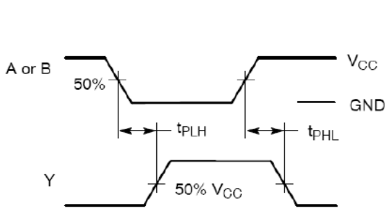
Figure 3. Switching Waveform
