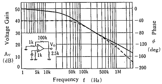
Voltage Gain, Phase vs. Frequency ( T_a = 25^\circ C , V^+/V^- = \pm 2.5V )
