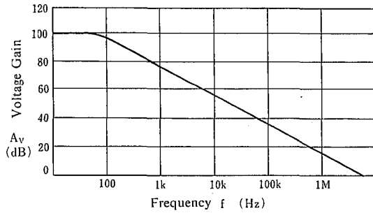
Voltage Gain vs. Frequency ( V^+/V^- = \pm 12.5V , T_a = 25^\circ C )
