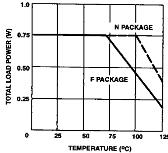
Total Load Power vs Temperature (NE591)
