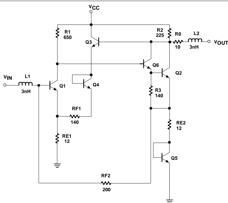
Figure 17. Schematic Diagram
