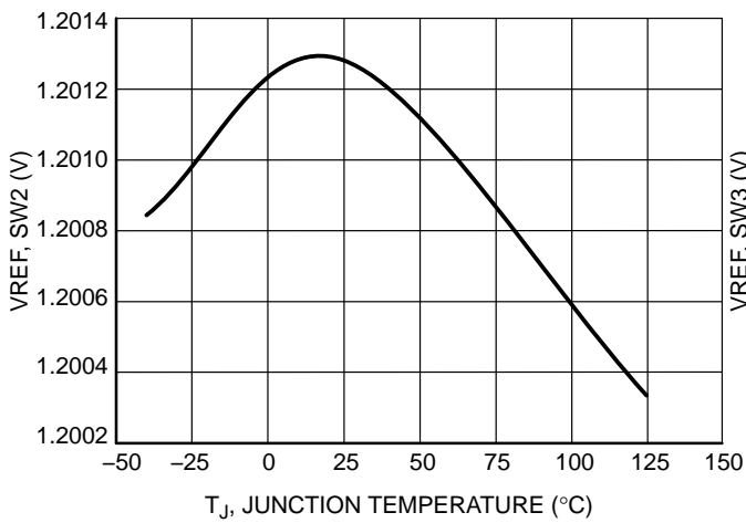
Figure 7. SW2 VREF vs. Junction Temperature
