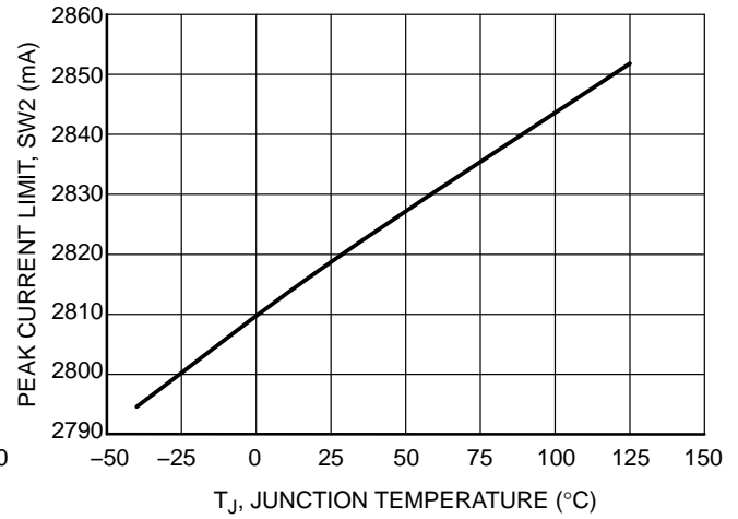
Figure 18. SW2 Peak Current Limit vs. Junction Temperature
