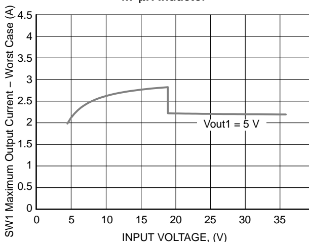
Figure 33. Switcher 1 Load Current Capability with a 2.2 \mu\text{H} Inductor
