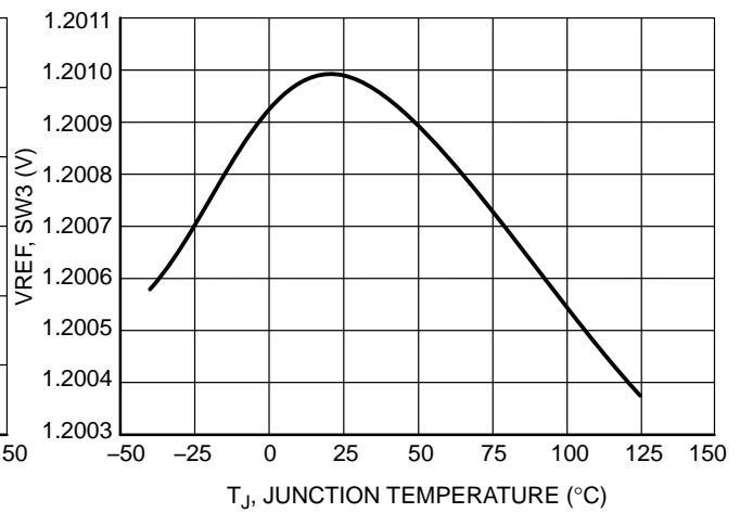
Figure 8. SW3 VREF vs. Junction Temperature
