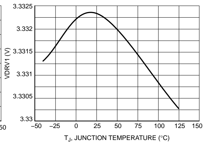
Figure 20. VDRV1 Voltage vs. Junction Temperature
