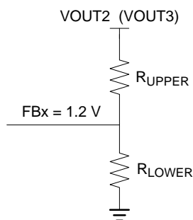
Figure 35. Output Voltage Selection with Feedback Divider
