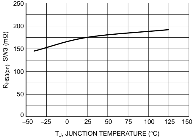
Figure 14. SW3 High Side R_{DS(on)} vs. Junction Temperature
