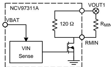
Figure 31. Internal Control for Minimum Load Circuit
