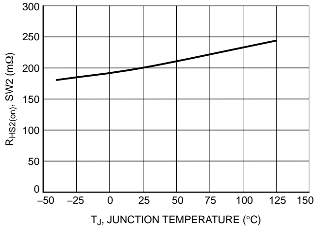
Figure 12. SW2 High Side R_{DS(on)} vs. Junction Temperature
