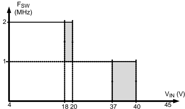
Figure 29. Switcher 1 Switching Frequency Reduction at High Input Voltage
