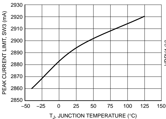
Figure 19. SW3 Peak Current Limit vs. Junction Temperature
