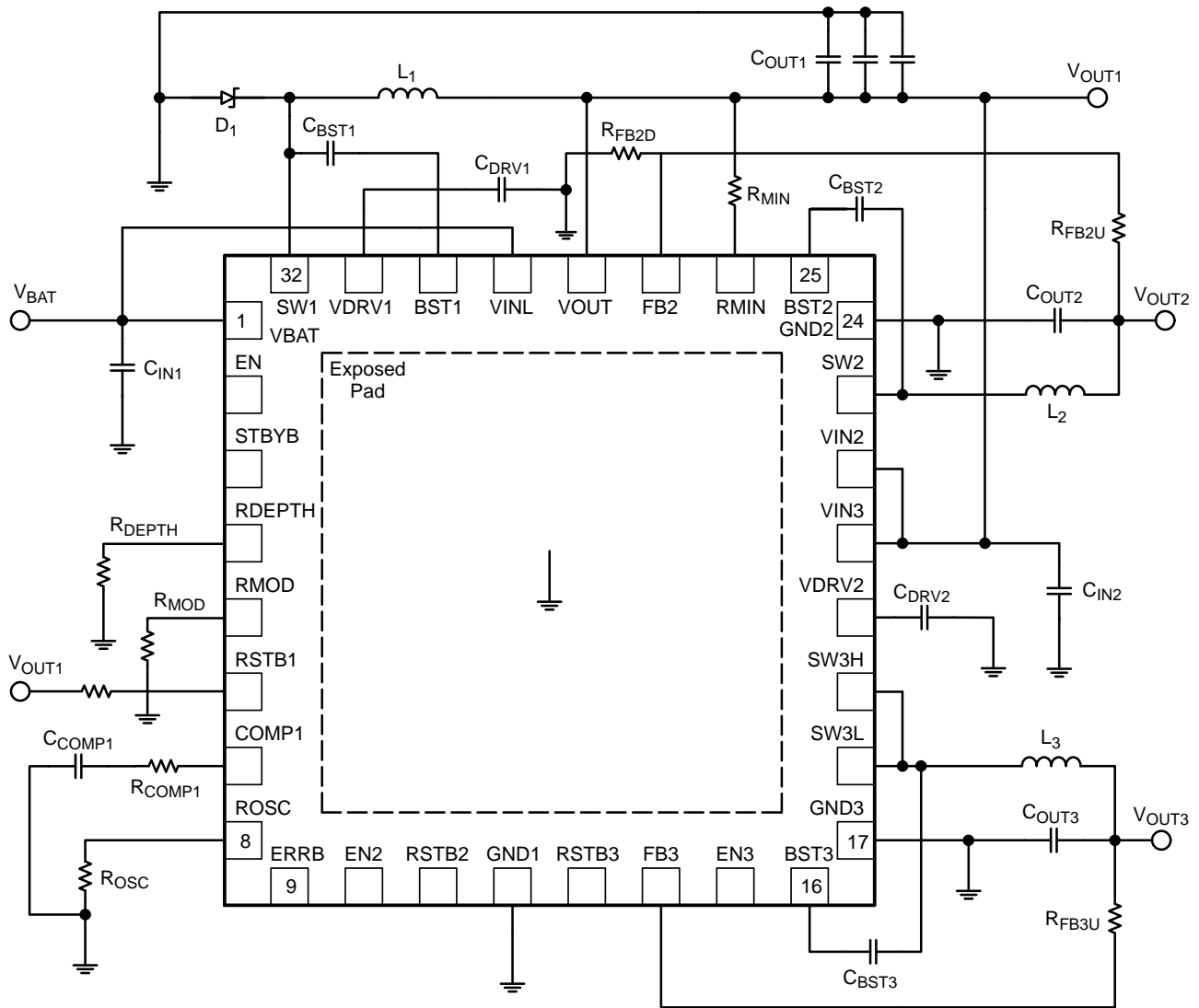
Figure 2. Typical Application – 5.0 V Version
