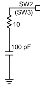
Figure 36. RC Snubber Circuit for Noise Performance at Heavy Loads
