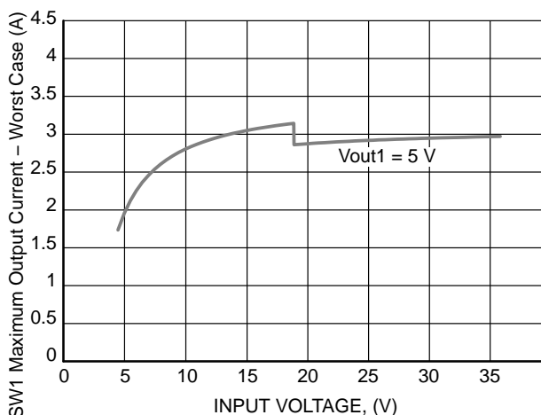
Figure 32. Switcher 1 Load Current Capability with a 4.7 \mu\text{H} Inductor
