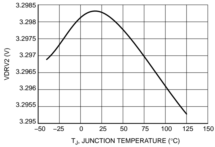
Figure 21. VDRV2 Voltage vs. Junction Temperature
