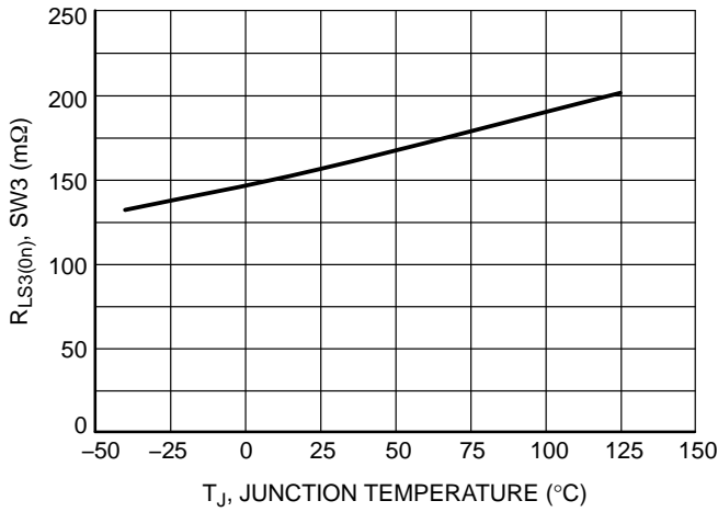
Figure 15. SW3 Low Side R_{DS(on)} vs. Junction Temperature
