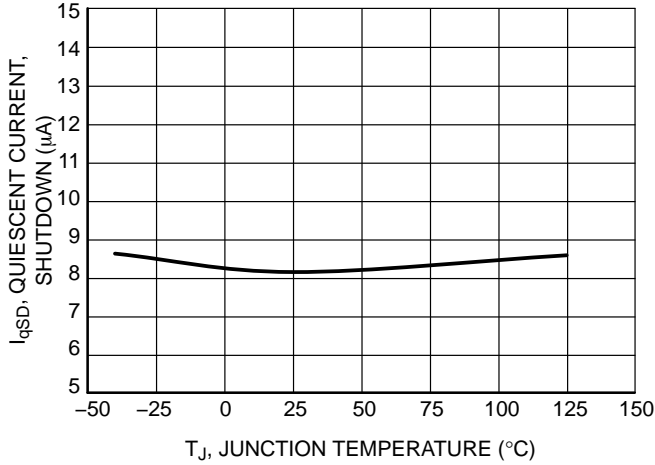
Figure 3. Quiescent Current (Shutdown) vs. Junction Temperature
