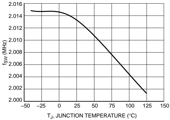
Figure 9. f_{sw} vs. Junction Temperature
