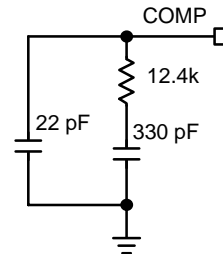
Figure 30. Recommended Compensation for Primary Switcher
