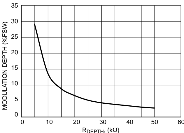
Figure 27. Modulation Depth vs. RDEPTH Value
