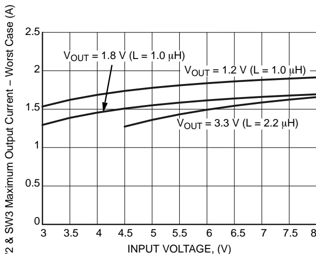
Figure 34. Switcher 2 or 3 Load Current Capability vs. Input Voltage
