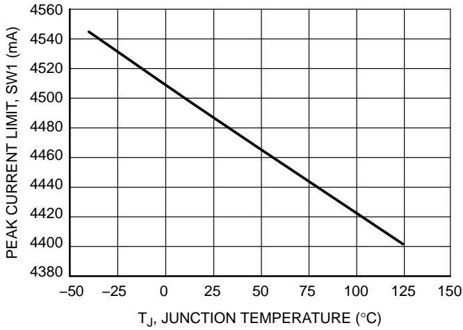
Figure 17. SW1 Peak Current Limit vs. Junction Temperature
