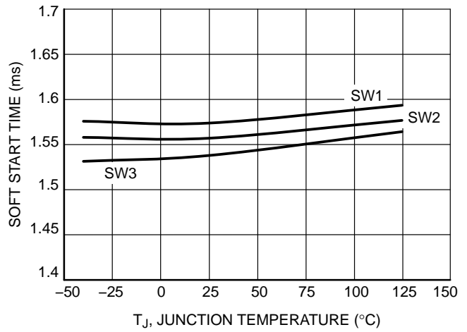
Figure 10. Soft Start Time vs. Junction Temperature
