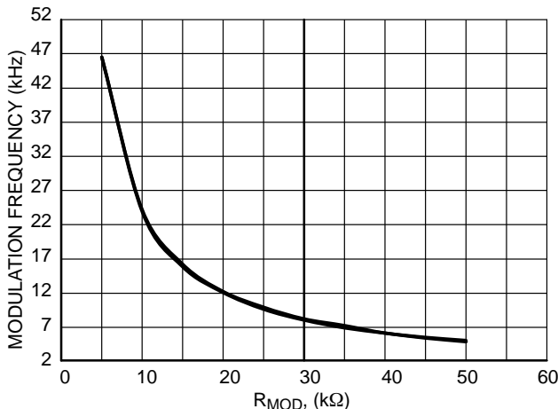
Figure 26. Modulation Frequency vs. RMOD Value
