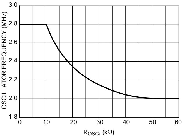
Figure 23. Oscillator Frequency vs. ROSC Value
