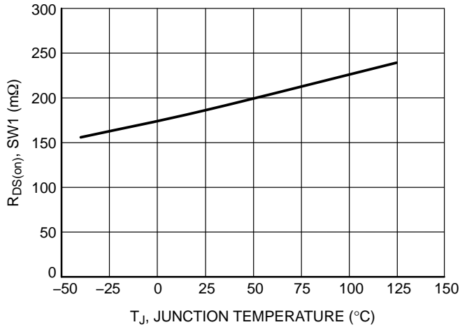
Figure 11. SW1 R_{DS(on)} vs. Junction Temperature
