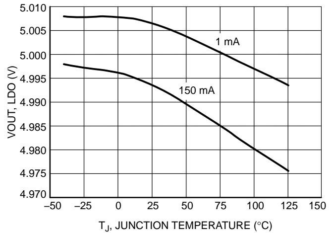
Figure 6. VOUT vs. Junction Temperature
