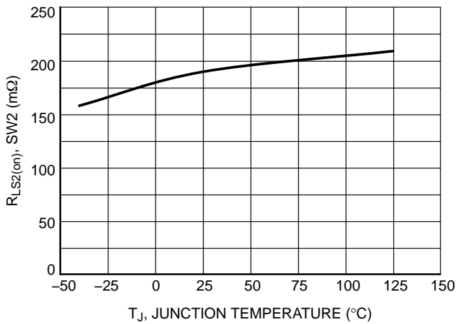
Figure 13. SW2 Low Side R_{DS(on)} vs. Junction Temperature
