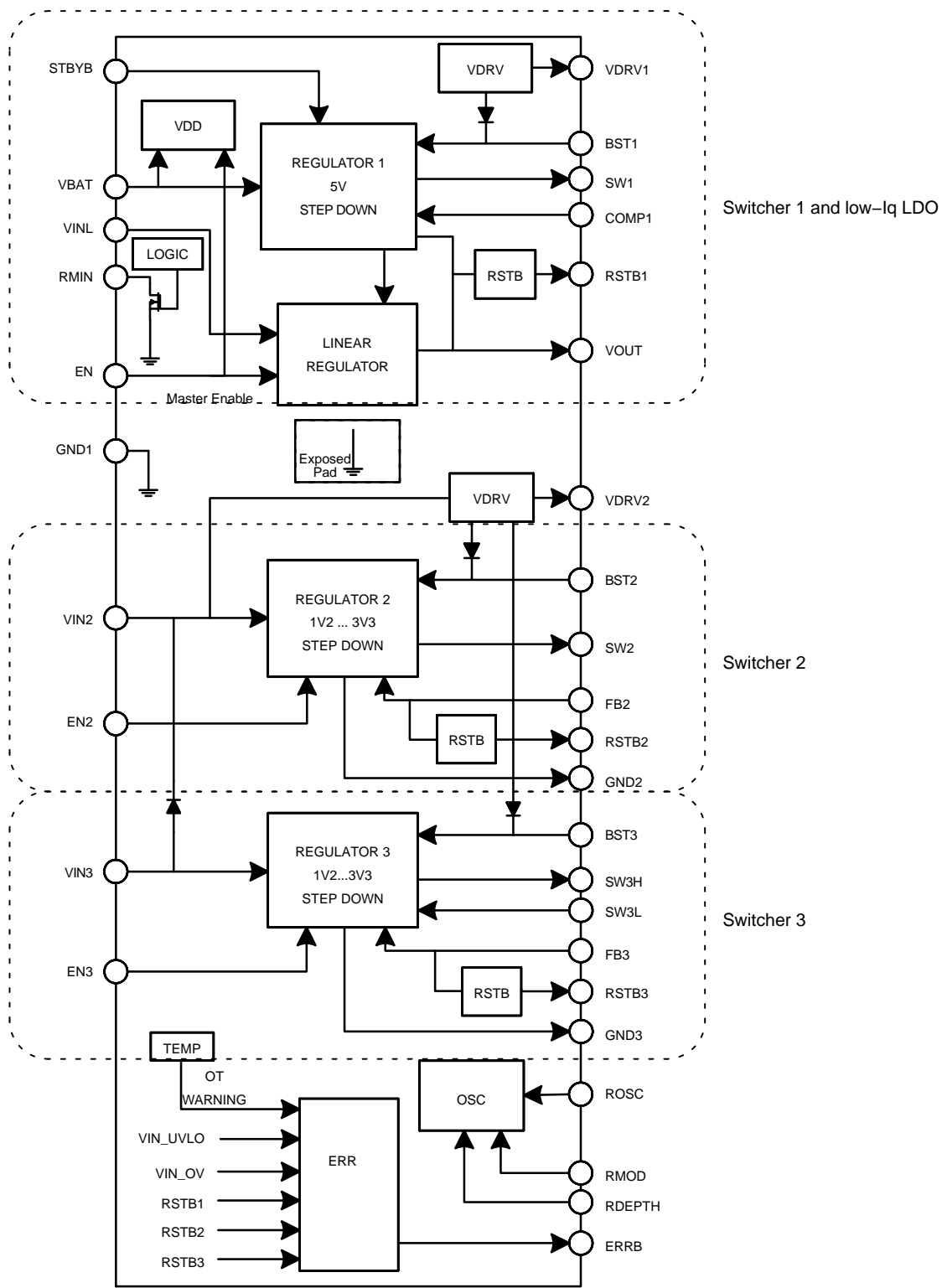
Figure 22. NCV97311A Block Schematic
