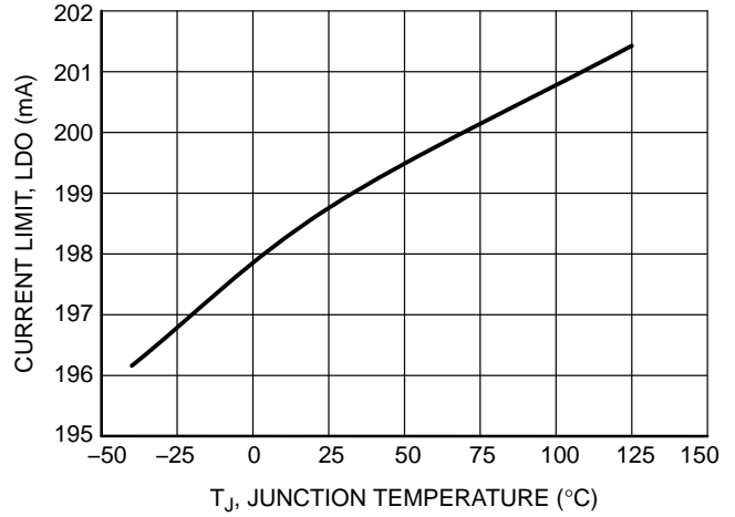
Figure 16. LDO Current Limit vs. Junction Temperature
