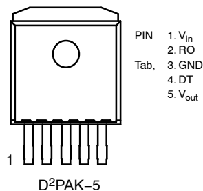
Figure 3. Pin Connections
