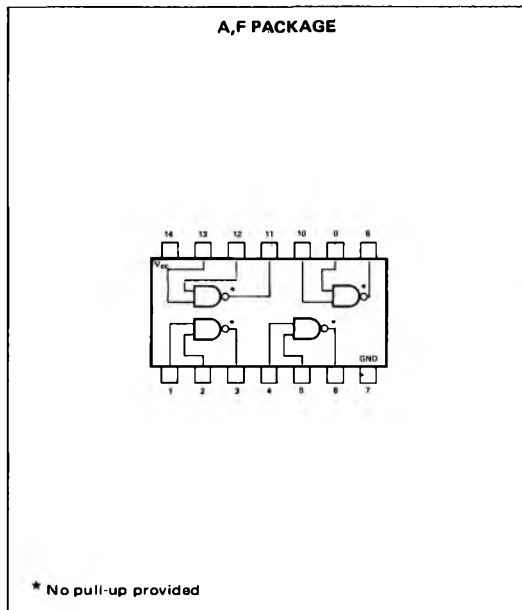
PIN CONFIGURATIONS
