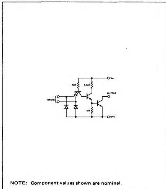
SCHEMATIC (each gate)
