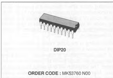
Figure 1 : Pin Connection.
