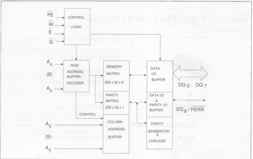
MK48H98/99 BLOCK DIAGRAM N° 1
