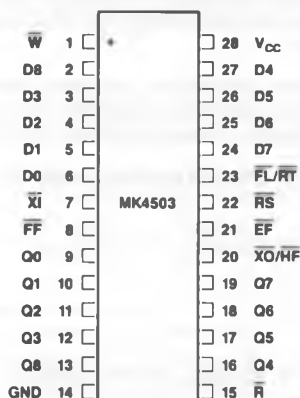
28 Pin Plastic DIP
