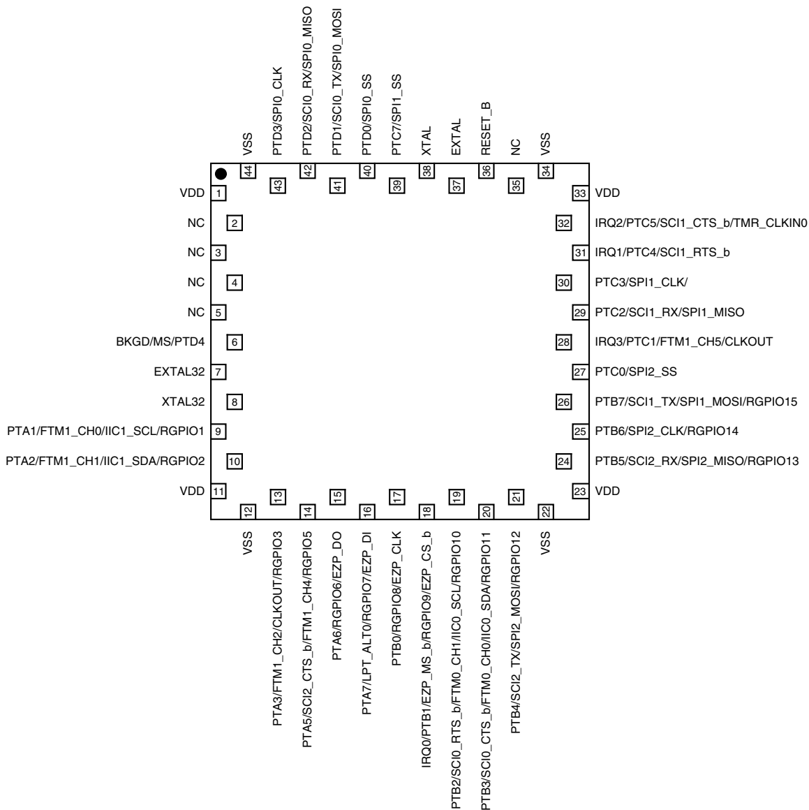
Figure 2. MCF51QW256 44-pin MAPLGA Pinout Diagram
