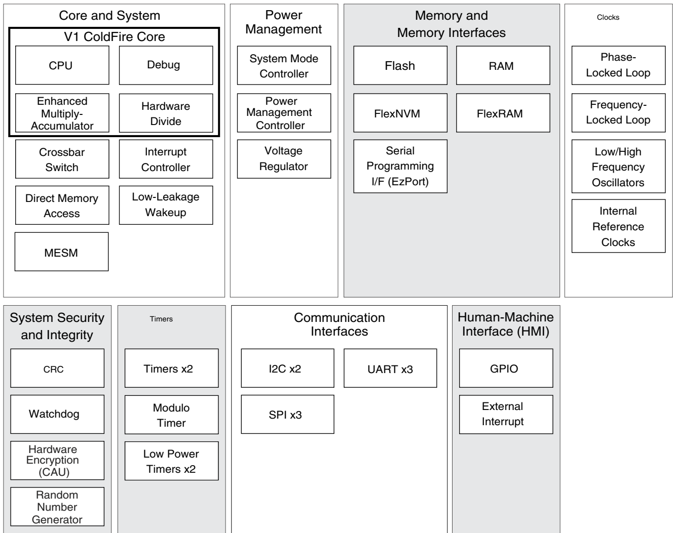
Figure 1. MCF51QW256 block diagram
