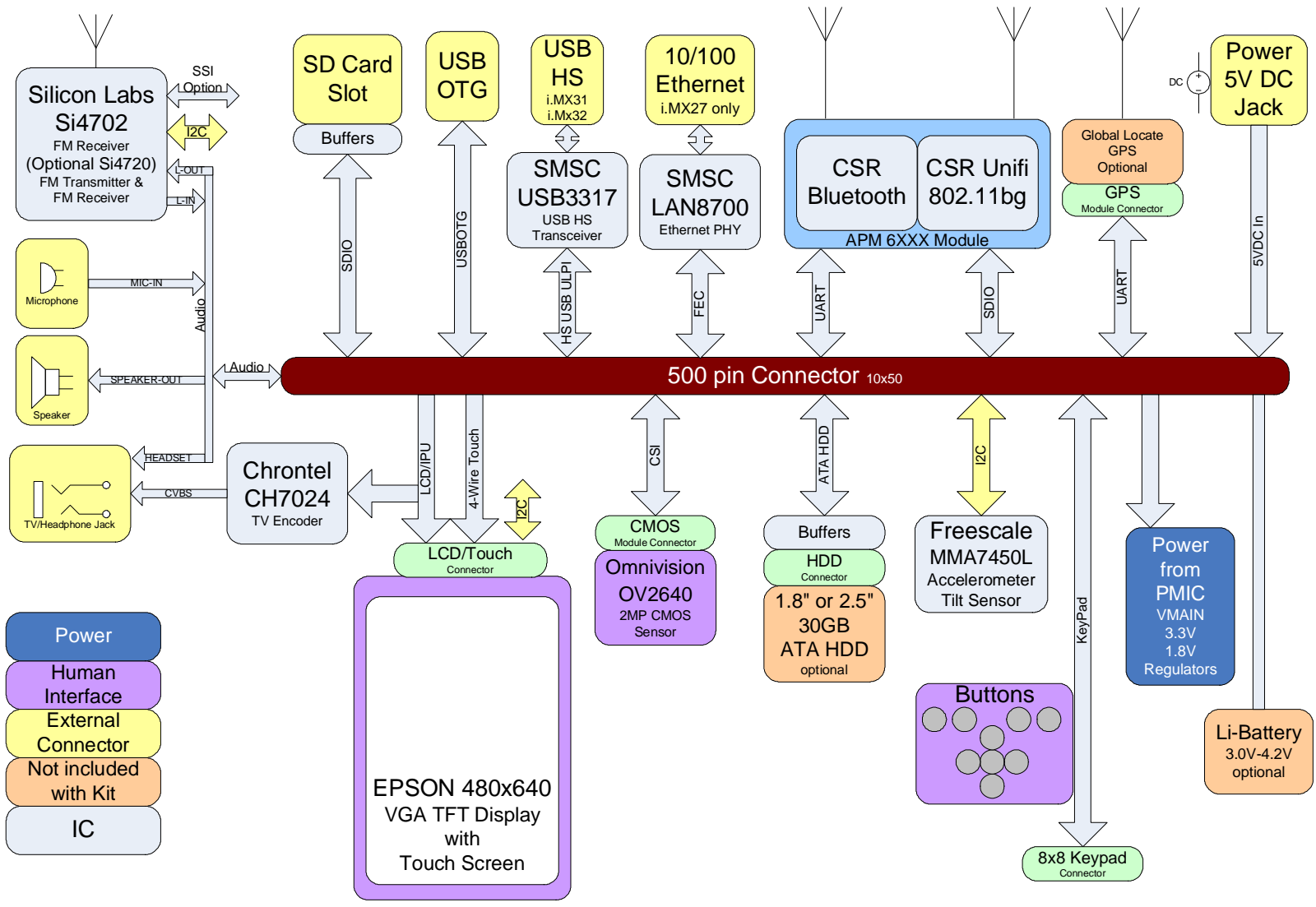
Figure 3 Personality Board Functional Block Diagram
