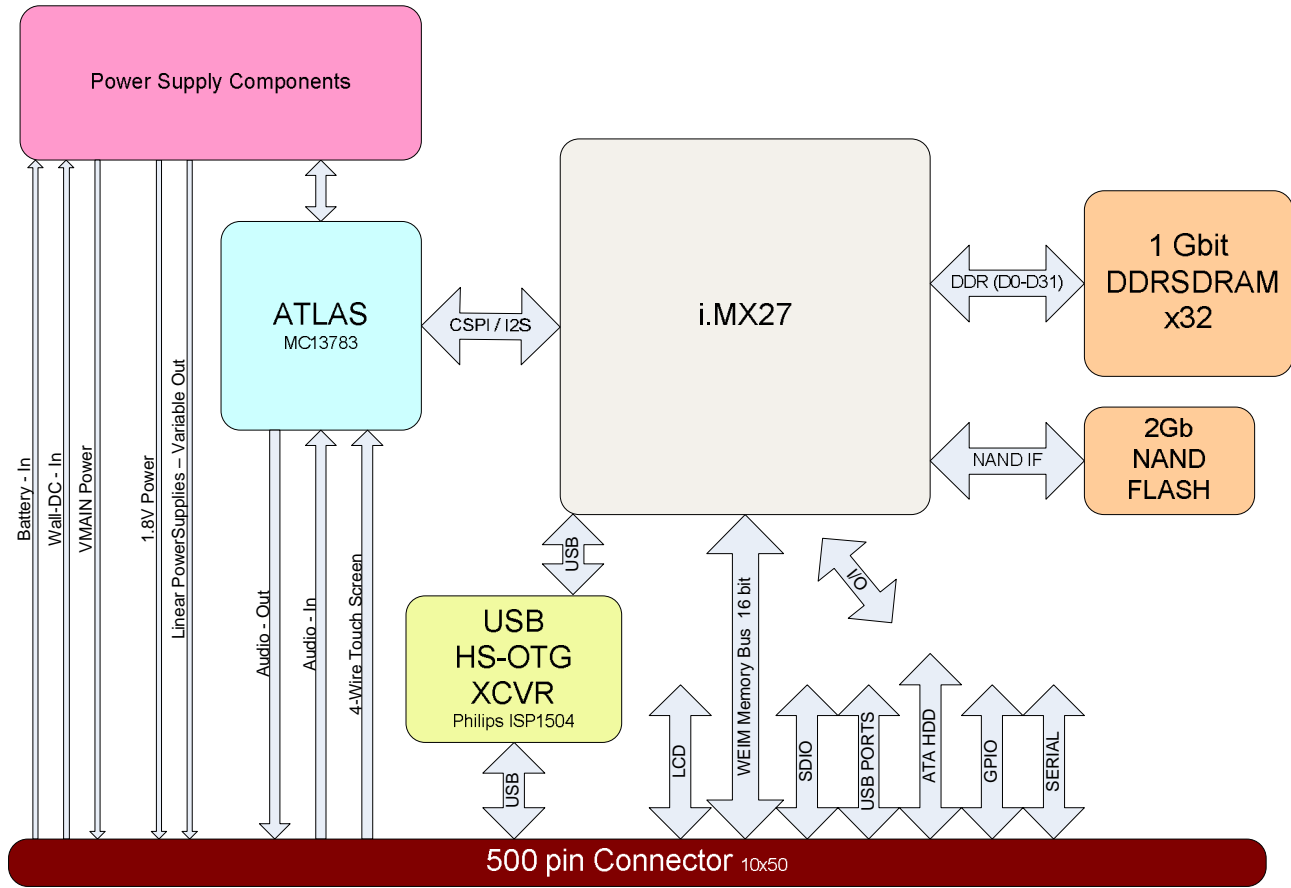
Figure 2 CPU Engine Board Block Diagram
