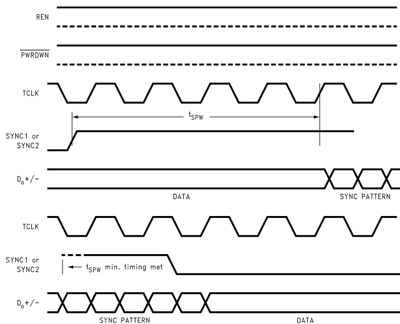
Figure 4. SYNC Timing Delays
