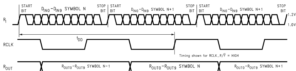
Figure 5. Deserializer Delay
