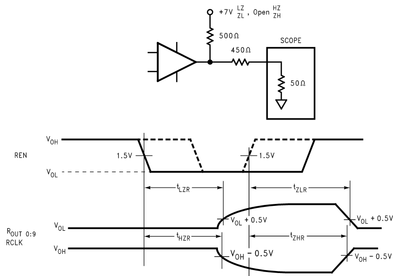
Figure 7. Deserializer TRI-STATE Test Circuit and Timing
