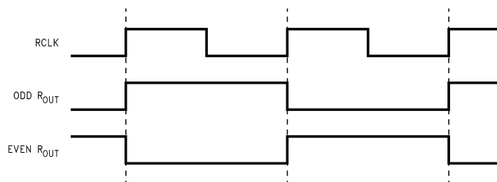
Figure 2. "Worst Case" Deserializer ICC Test Pattern
