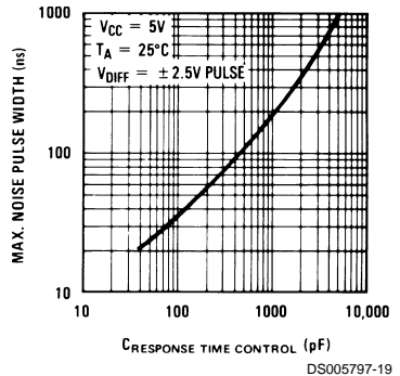
Noise Rejection
