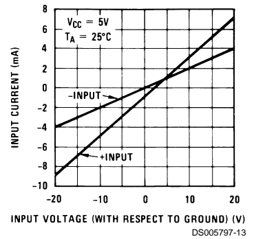
Input Characteristics
