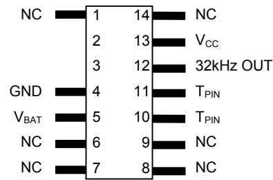
DS32kHz 14-Pin DIP Module (300-mil)
