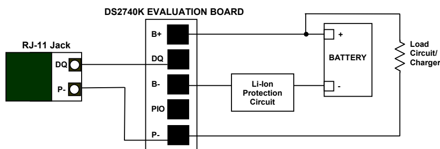
Figure 1. PD122402 Cell, Load, and Charger Connections
