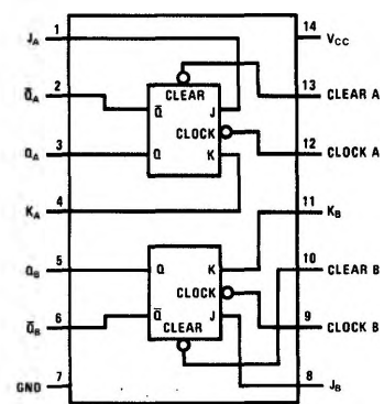
DM54107/DM74107
