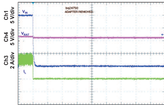
CHARGER ON ADAPTER REMOVAL
