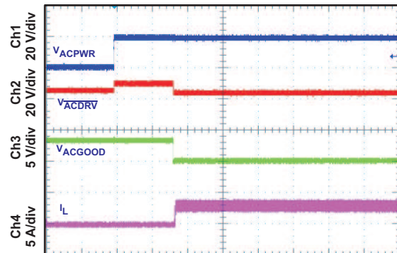
SYSTEM SELECTOR ON ADAPTER INSERTION
