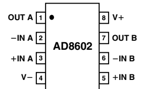
8-Lead MSOP (RM Suffix)
