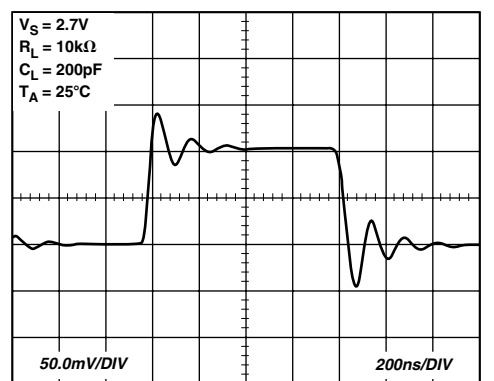
TPC 42. Small Signal Transient Response
